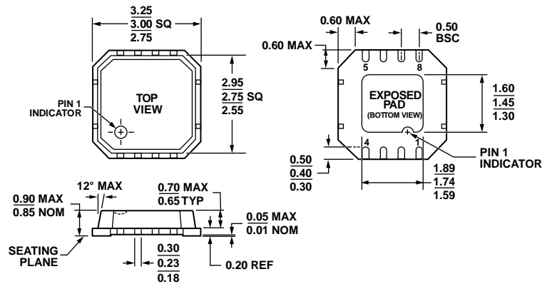
Figure 44. 8-Lead Frame Chip Scale Package [LFCSP_VD] 3 mm × 3 mm Body, Very Thin, Dual Lead (CP-8-2) Dimensions shown in millimeters
