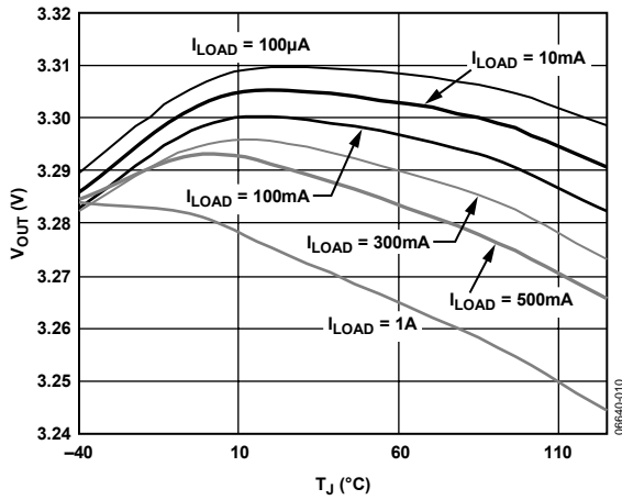
Figure 10. Output Voltage vs. Junction Temperature
