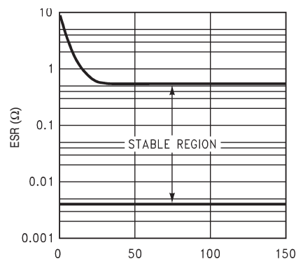
Figure 31. 2.2- \mu\text{F} /3.3- \mu\text{F} Stable ESR Range for Output Voltage \geq 2.5 V
