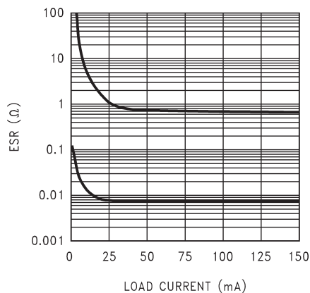
Figure 29. 2.2- \mu\text{F} Stable ESR Range for Output Voltage \leq 2.3 V
