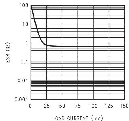
Figure 30. 4.7- \mu\text{F} Stable ESR Range for Output Voltage \leq 2.3 V
