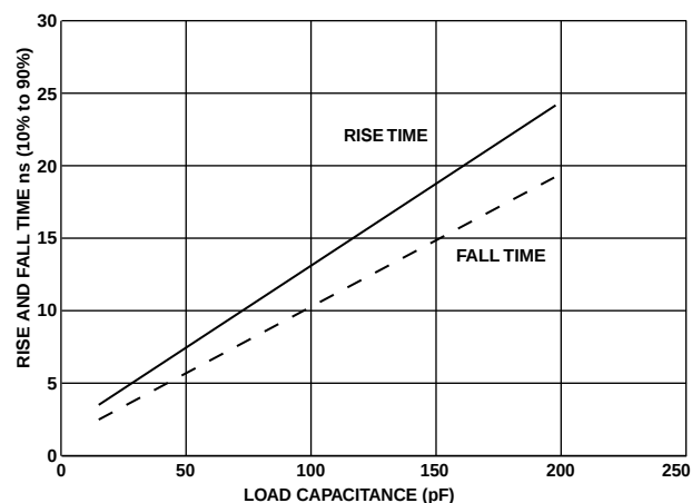
Figure 52. Typical Rise and Fall Times (10% to 90%) versus Load Capacitance for Driver C at V_{DDEXT} = 2.25\text{ V}
