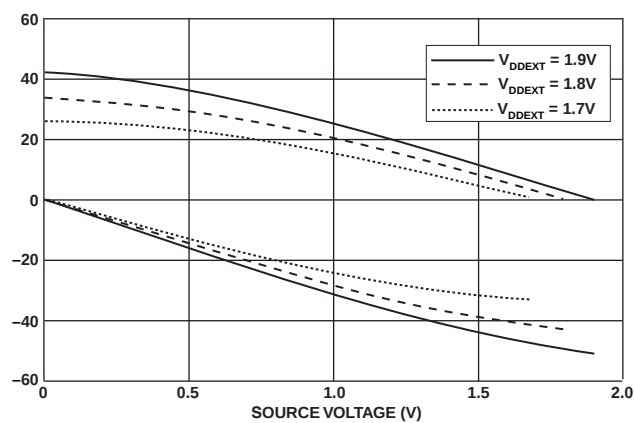
Figure 40. Drive Current D ( V_{DDEXT} = 1.8 \text{ V} )
