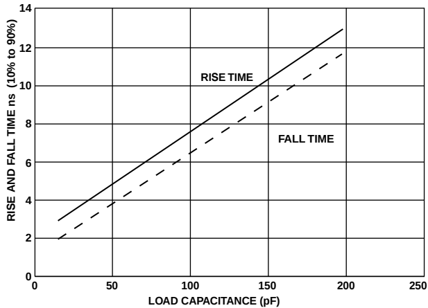
Figure 56. Typical Rise and Fall Times (10% to 90%) versus Load Capacitance for Driver D at V_{DDEXT} = 3.65\text{ V}
