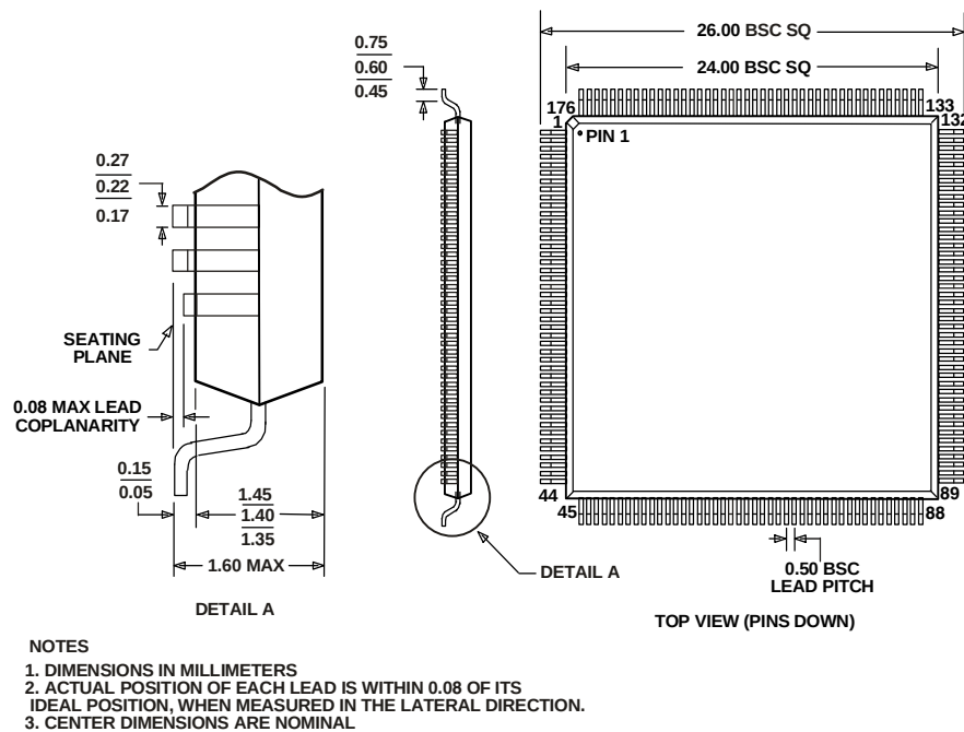
Figure 61. 176-Lead Low Profile Quad Flat Package (LQFP) ST-176-1
