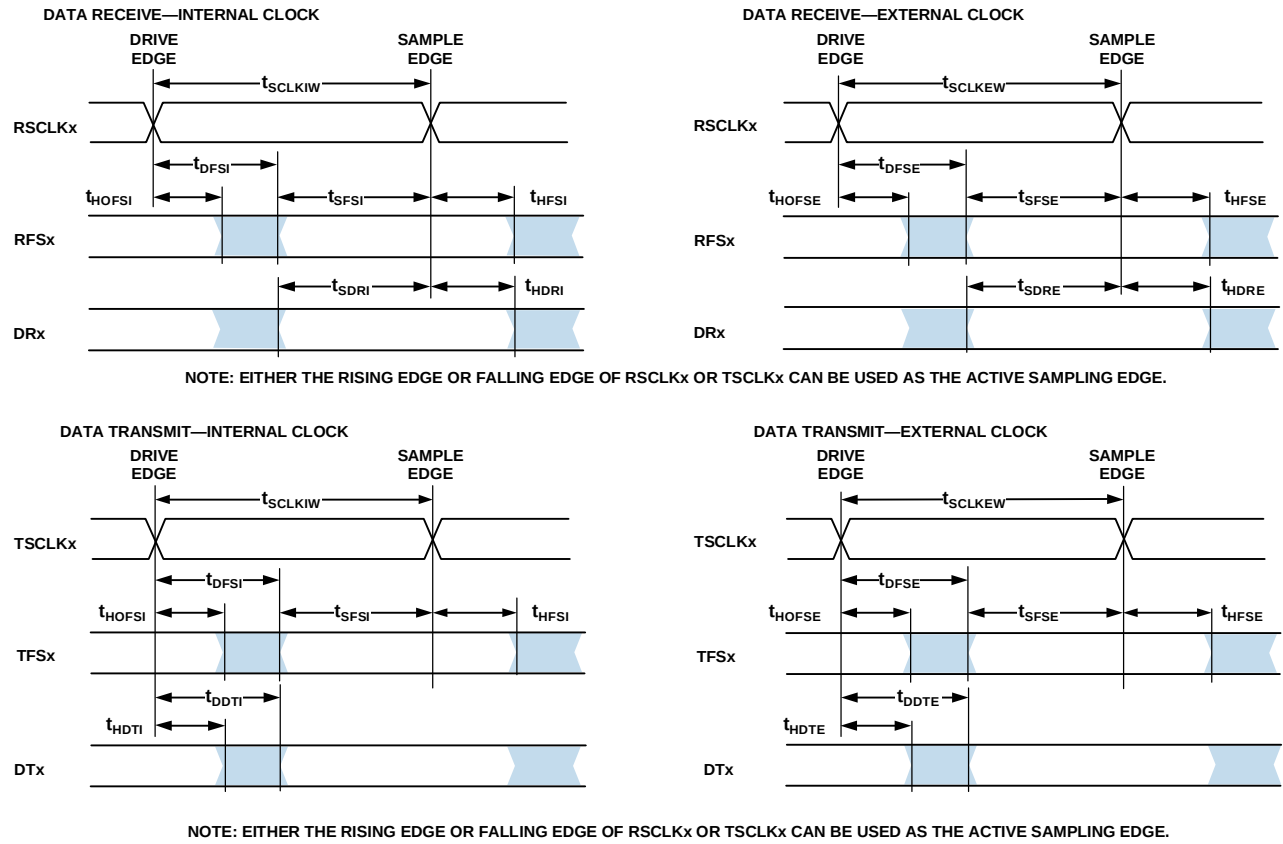
Figure 22. Serial Ports
