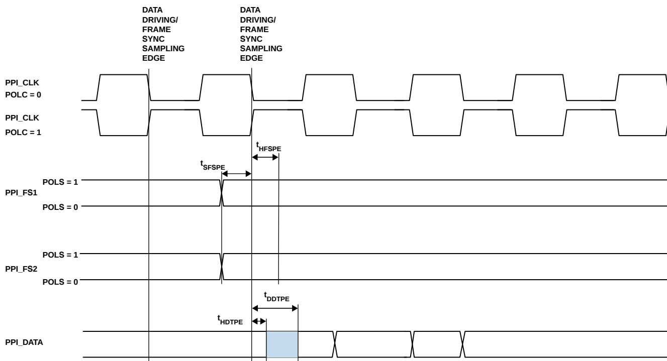
Figure 21. PPI GP Tx Mode with External Frame Sync Timing (Bit 8 of PPI_CONTROL Set)
