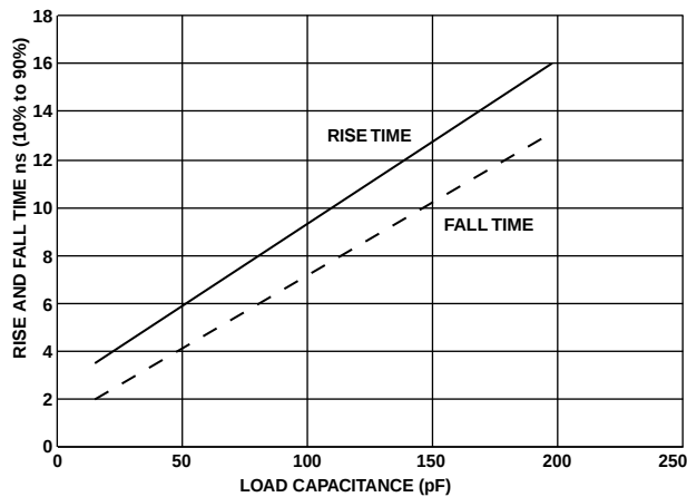
Figure 55. Typical Rise and Fall Times (10% to 90%) versus Load Capacitance for Driver D at V_{DDEXT} = 2.25\text{ V}
