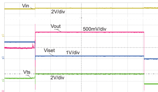
Figure 9. Battery Removal - GND Removed 1st, 42- \Omega Load
