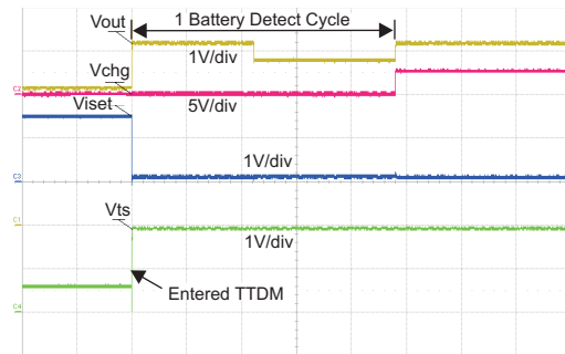
Figure 10. Battery Removal with OUT and TS Disconnect 1st, With 100- \Omega Load
