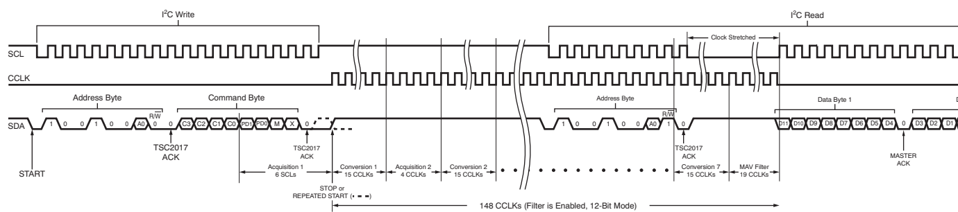
Figure 33. Data Acquisition Cycle (Filter Enabled)
