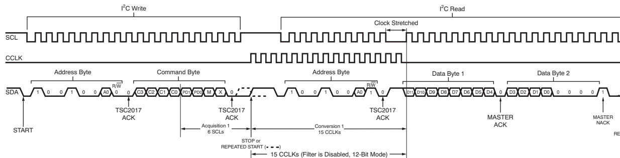
Figure 34. Data Acquisition Cycle (Filter Disabled)
