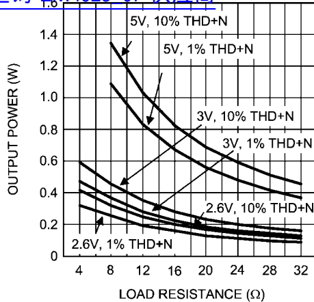
Output Power vs Load Resistance 查询"LM4923_07"供应商
