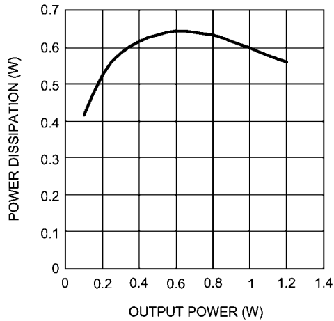
Power Dissipation vs Output Power 查询"LM4923_07"供应商 V_{DD} = 5V , R_L = 8\Omega
