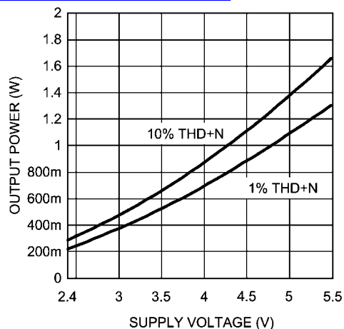
Output Power vs Supply Voltage 查询"LM4923_01"供应商
