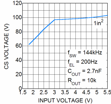
Peak Output Voltage vs. Input Voltage
