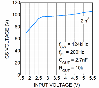
Peak Output Voltage vs. Input Voltage
