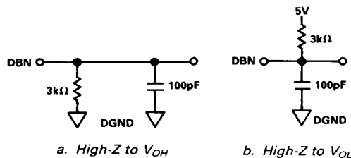
Figure 1. Load Circuits for Data Access Time Test
