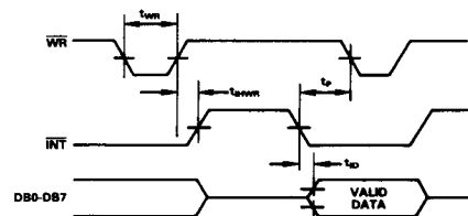
Figure 6. WR-RD Mode Stand-Alone Operation, \overline{\text{CS}} = \overline{\text{RD}} = 0
