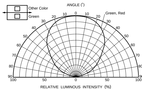
Fig. 2 Directional pattern (2)
