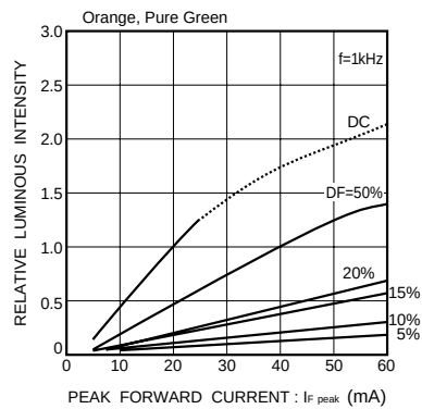
Fig. 33 Luminous intensity vs. peak forward current
