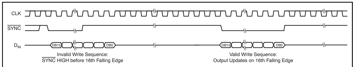
Figure 104. DAC8311 \overline{\text{SYNC}} Interrupt Facility
