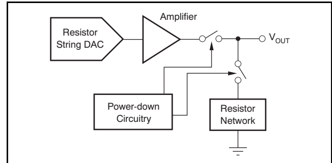
Figure 106. Output Stage During Power-Down
