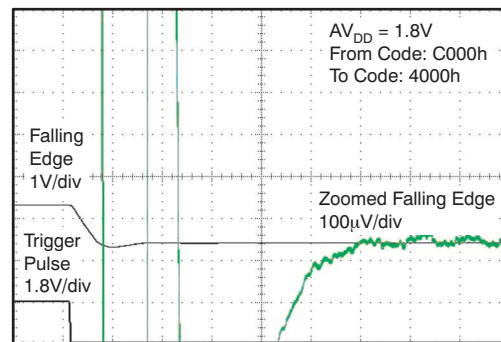
HALF-SCALE SETTling TIME 1.8V FALLING EDGE
