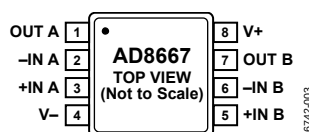
Figure 3. 8-Lead MSOP (RM-8), 8-Lead SOIC (R-8)
