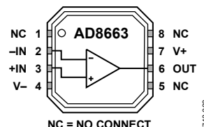
Figure 2. 8-Lead LFCSP (CP-8-2)
