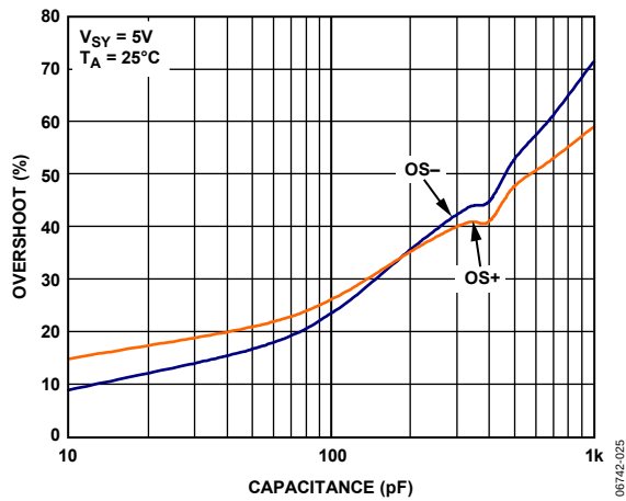
Figure 25. Small-Signal Overshoot vs. Load Capacitance, V_{SV} = 5\text{ V}
