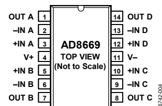
Figure 4. 14-Lead SOIC (R-14), 14-Lead TSSOP (RU-14)
