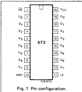
Fig. 1 Pin configuration.
