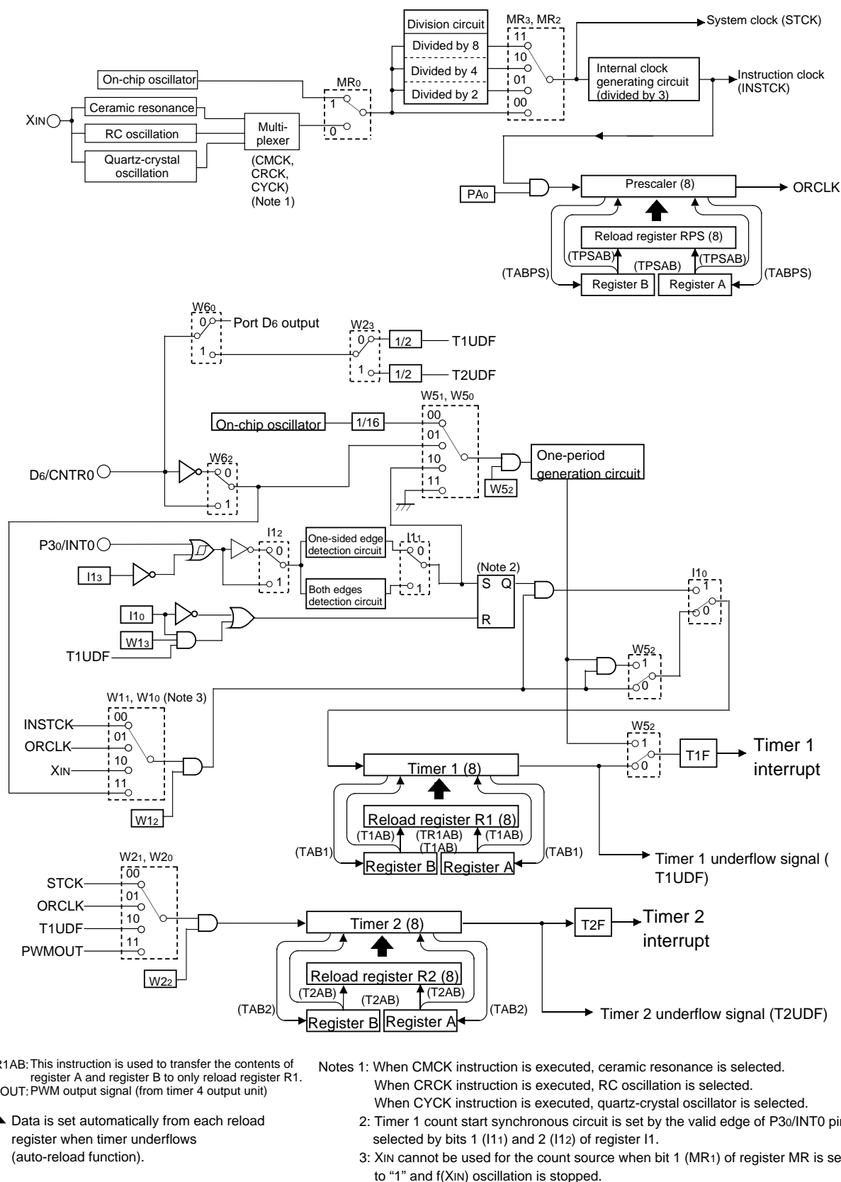
Fig. 25 Timer structure (1)
