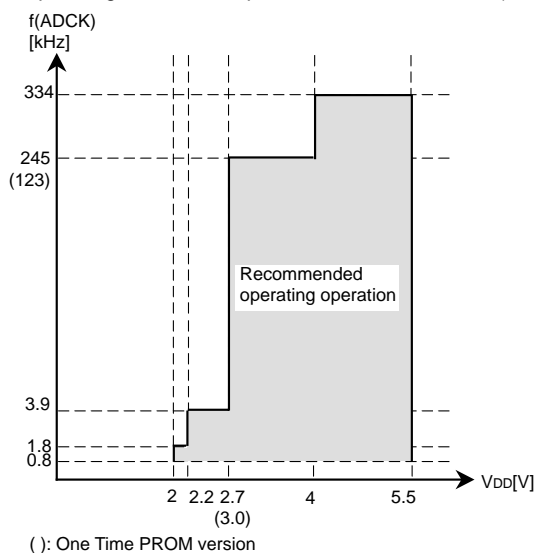
&lt;Operating condition map of A/D conversion clock (ADCK) &gt;
