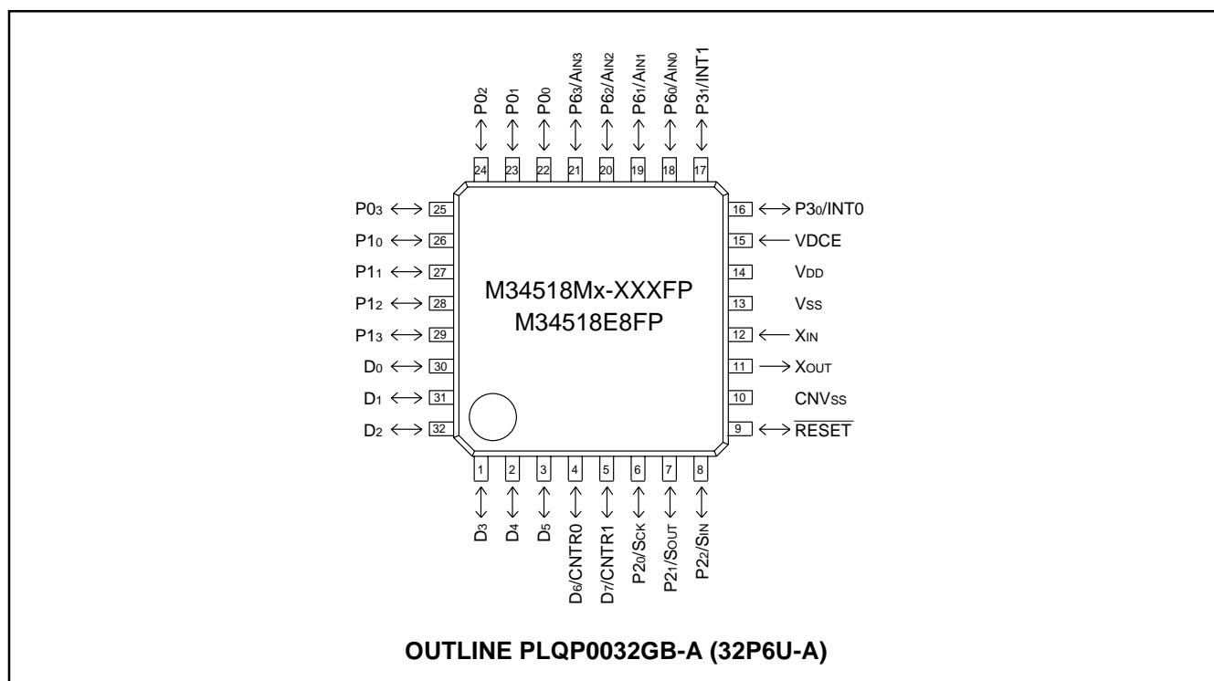
Pin configuration (top view) (4518 Group)
