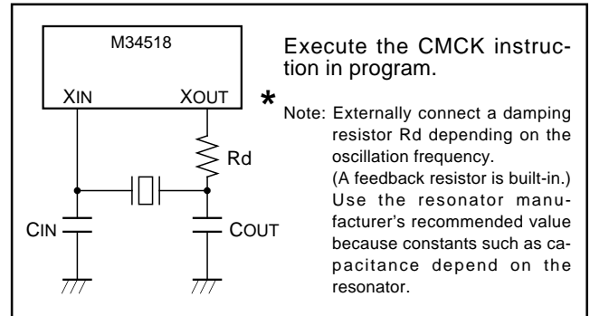
Fig. 59 Ceramic resonator external circuit
