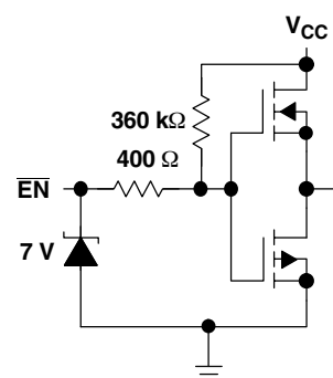
ACTIVE-LOW ENABLE
