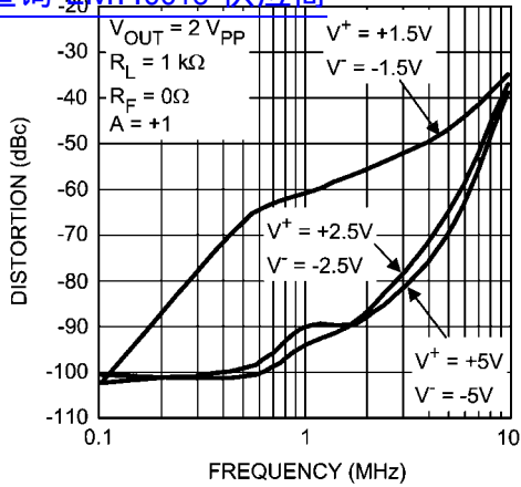
HD3 vs. Frequency and Supply Voltage 查询"LMH6618"供应商
