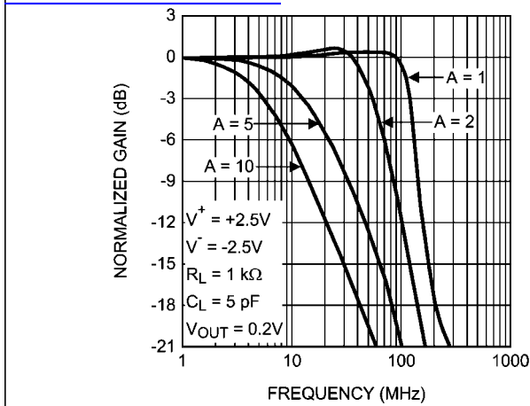
Closed Loop Gain vs. Frequency for Various Gains
