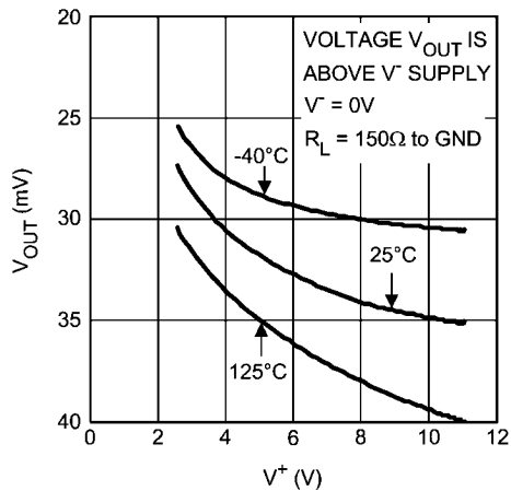
V_{OUT} vs. V^+
