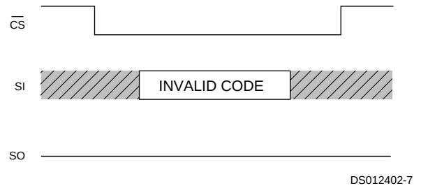
FIGURE 5. Invalid Op-Code
