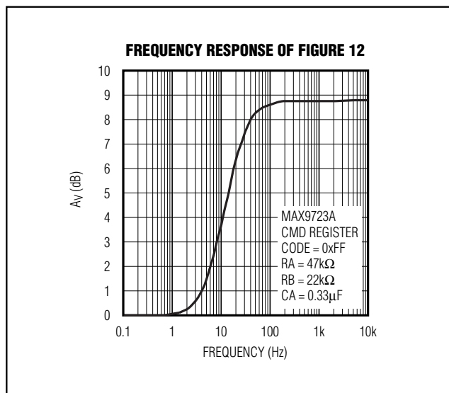
Figure 13. Increasing the Maximum Gain Using BassMax
