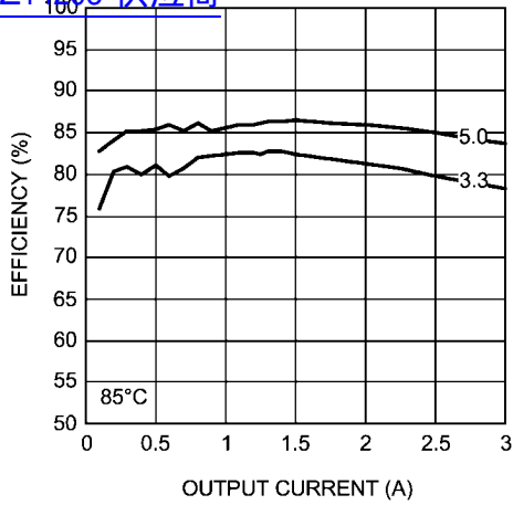
Efficiency 36V input @ 85°C 查询"LMZ14203"供应商
