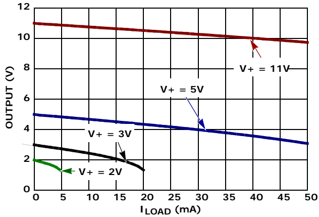
FIGURE 9. COMPARATOR OUTPUT HIGH VOLTAGE vs LOAD
