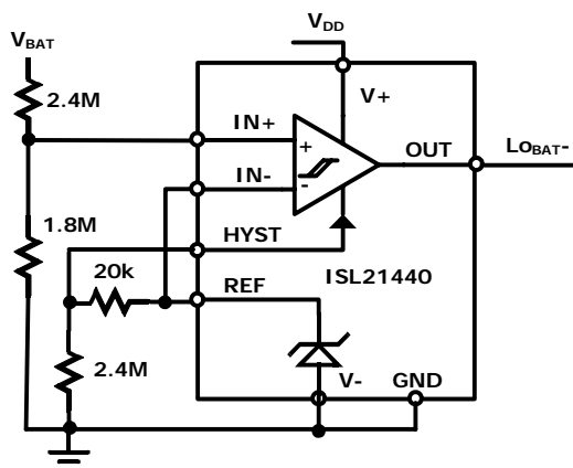
FIGURE 24. LOW BATTERY DETECTOR WITH HYSTERESIS
