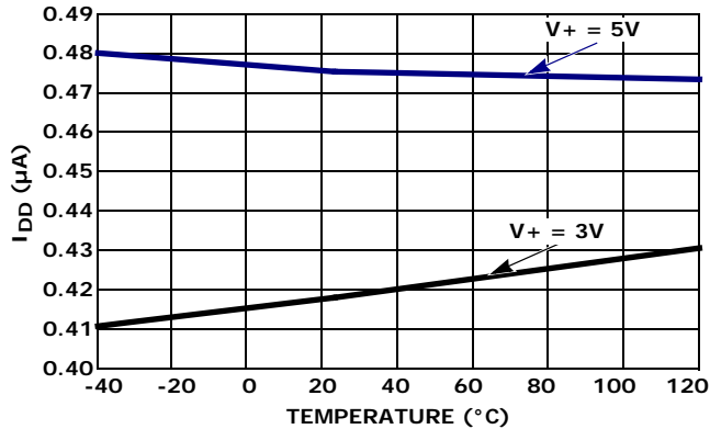
FIGURE 1. I_{DD} vs TEMPERATURE
