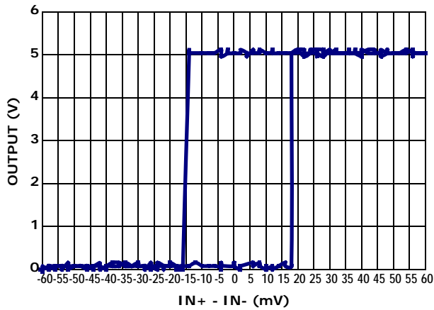
FIGURE 11. HYSTERESIS - 12.5mV ( V_+ = 5V )
