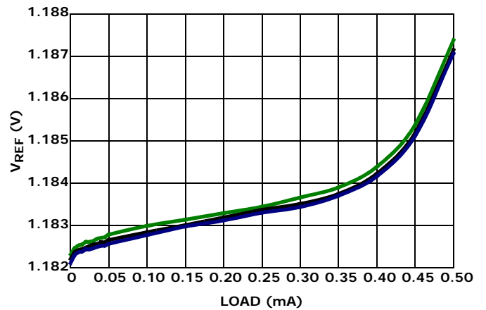
FIGURE 6. V_{REF} vs LOAD (SINK)
