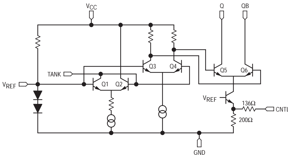
Figure 1. Simplified Schematic
