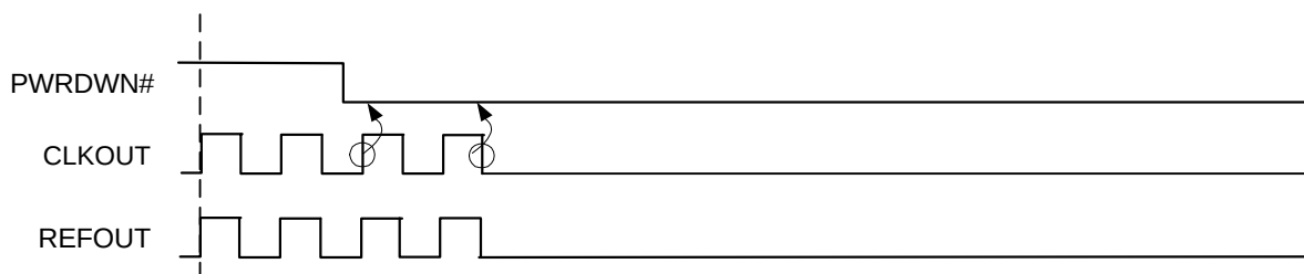
Figure 1. Power-down Assertion
