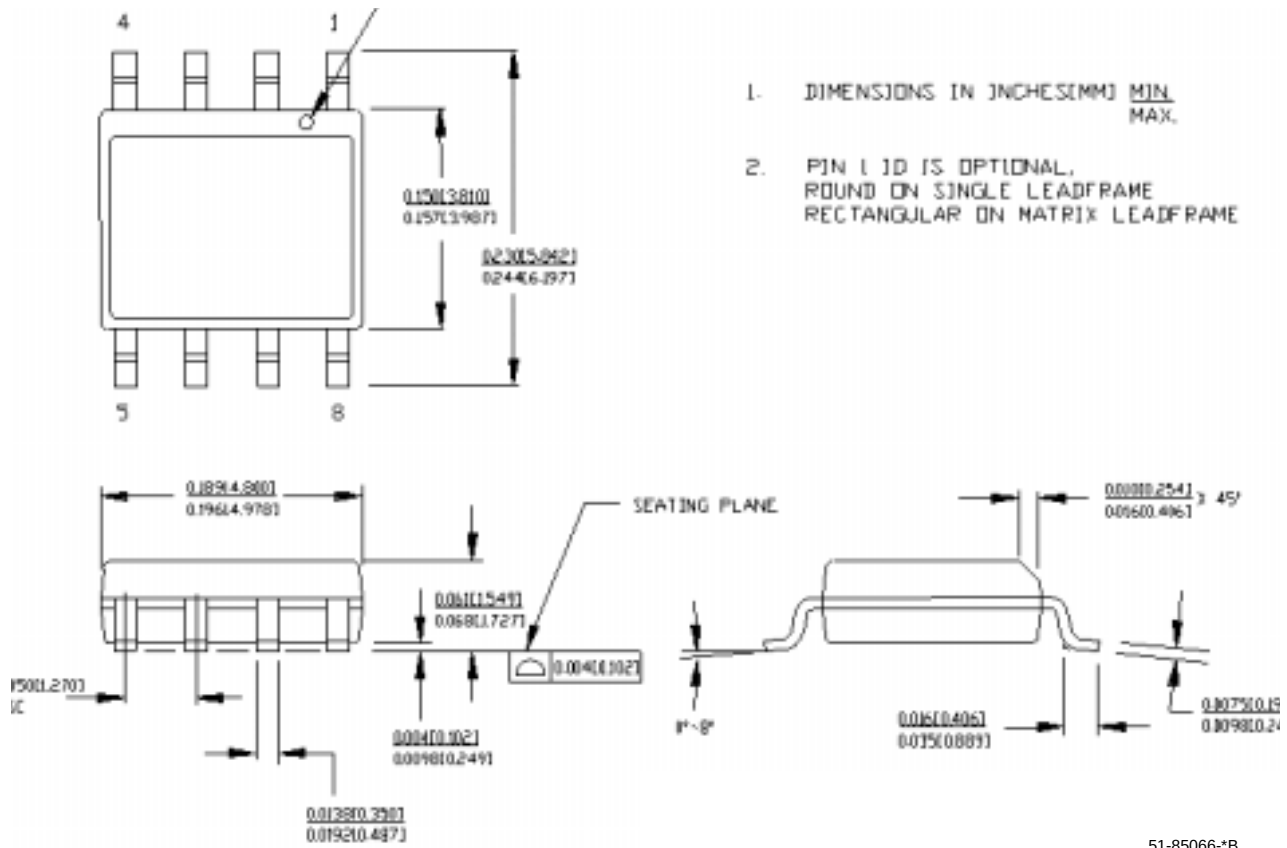
8-lead (150-Mil) SOIC – S8
