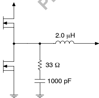
Figure 35. Filter Components
