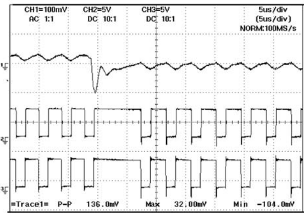
Figure 33. 15 A Load Transient Waveforms
