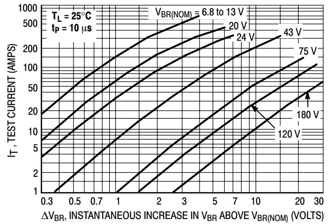
Figure 6. Dynamic Impedance
