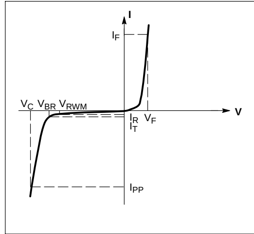
Uni-Directional TVS
