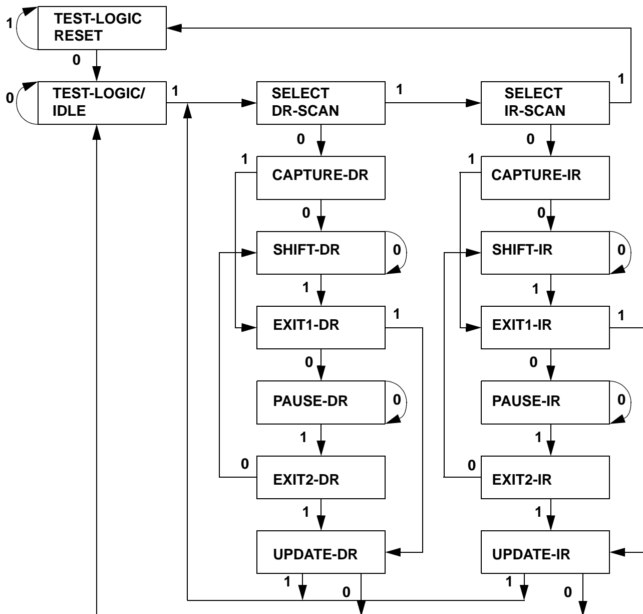
TAP Controller State Diagram [10]
