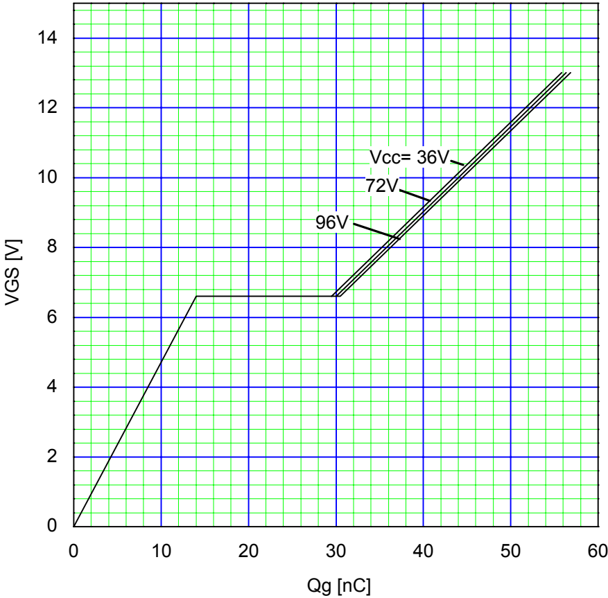
Typical Gate Charge Characteristics V GS =f(Q g ):I D =25A,T ch =2°C
