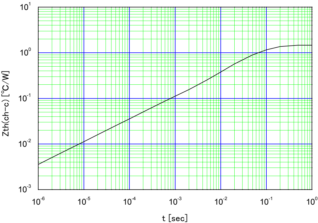
Transient Thermal Impedance Z_{th(ch-c)}=f(t):D=0
