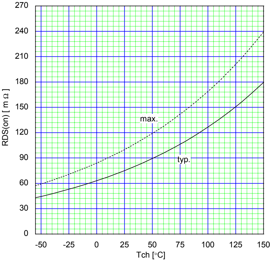
Drain-Source On-state Resistance R_{DS(on)}=f(T_{ch}) : I_D=12.5\text{A} , V_{GS}=10\text{V}
