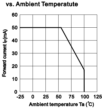
Fig.1 Forward Current
