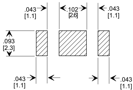
MOUNTING PATTERN
