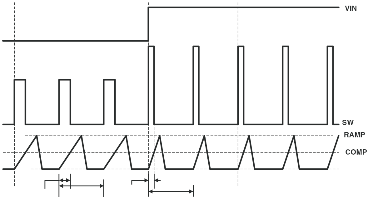
Figure 2. Voltage Feed-Forward Effect on PWM Duty Cycle
