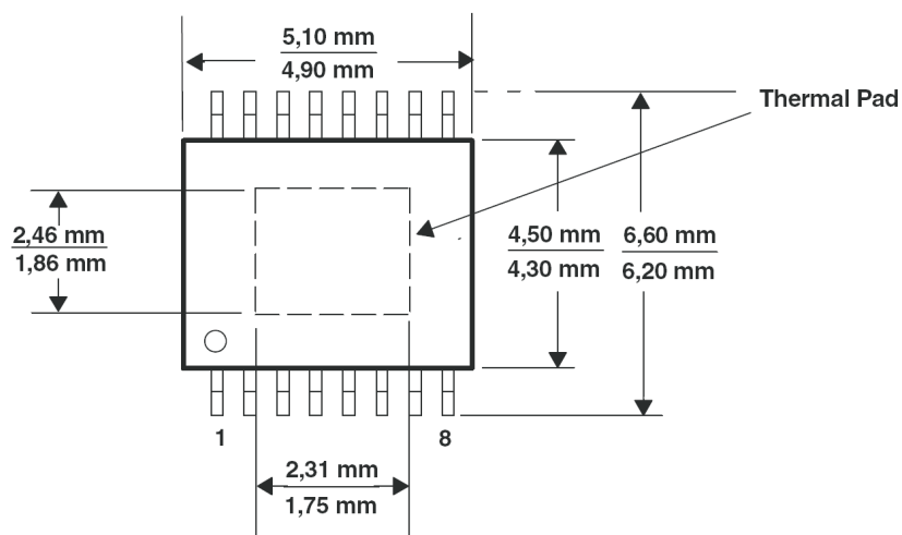
Figure 16. PowerPAD Dimensions
