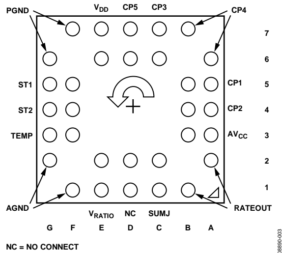
Figure 3. Pin Configuration
