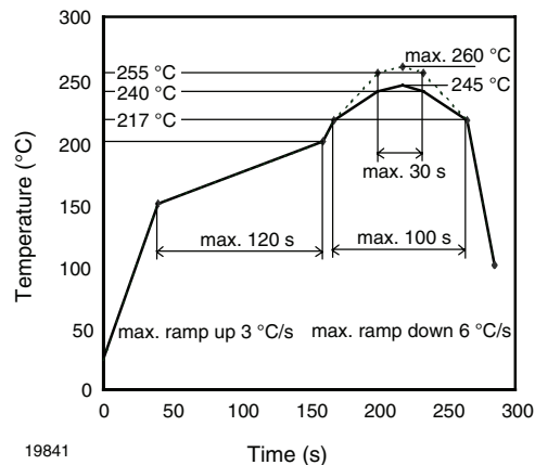
Fig. 9 - Lead (Pb)-free Reflow Solder Profile acc. J-STD-020
