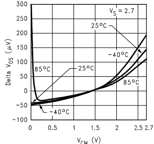
Delta V_{OS} vs. V_{CM} (Ref V_{CM} = 1.35V )
