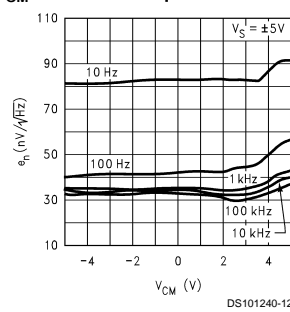
Voltage Noise vs. V_{CM} @ Various Frequencies
