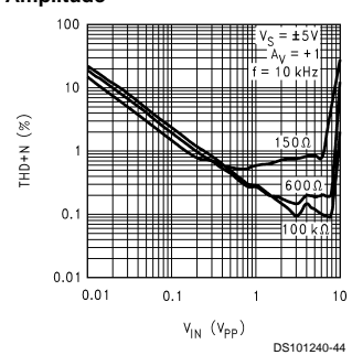
THD+N vs. Amplitude
