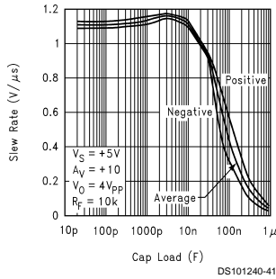
Slew Rate vs. Capacitive Load
