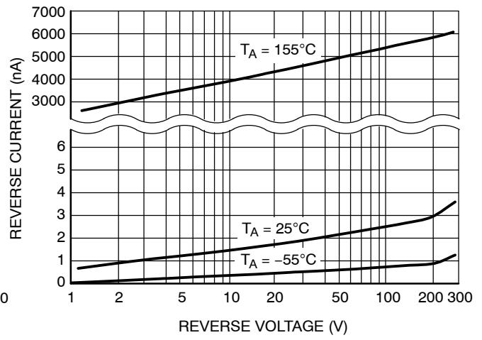
Figure 3. Reverse Leakage
