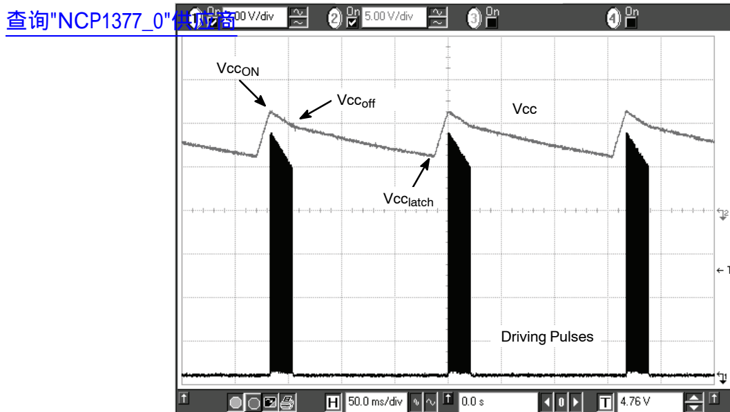
Figure 28. Typical Waveforms in Short Circuit Conditions
