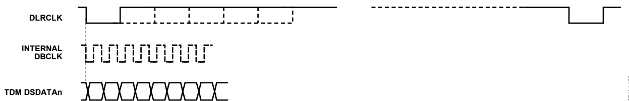
Figure 30. I²S Pipeline Mode in DAC Serial Data Transmission (Applicable in Stereo and TDM, Useful for High Frequency TDM Transmission; This Mode Is Also Available in the ADC Serial Data Port)
