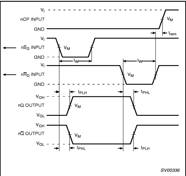
Figure 2.The set (nSD) and reset (nRD) input to output (nQ, nQ̄) propagation delays, the set and reset pulse widths and the nRD to nCP removal time
