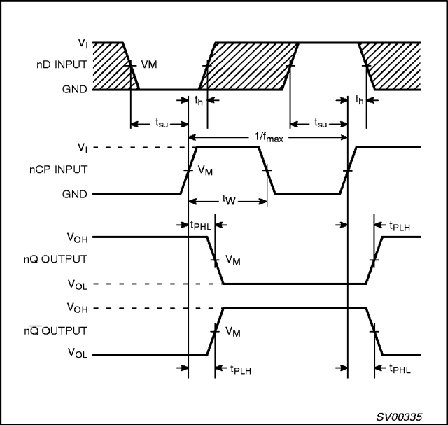
Figure 1.The clock (nCP) to output (nQ, nQ̄) propagation delays, the clock pulse width, the nD to nCP setup times, the nCP to nD hold times, the output transition times and the maximum clock pulse frequency
