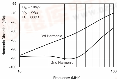
Differential Harmonic Distortion
