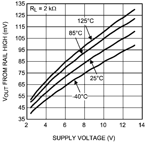
Output Swing High vs. Supply Voltage 查询"LMV842"供应商 R_L = 2\text{k}\Omega
