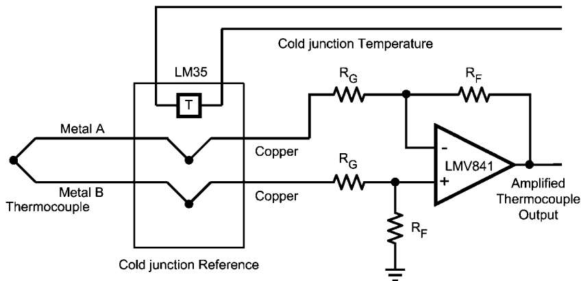
FIGURE 9. Thermocouple Amplifier
