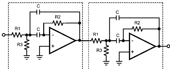
FIGURE 4. Active Filter
