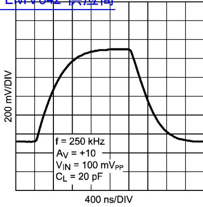
Large Signal Step Response with Gain = 10 查询"LMV842"供应商
