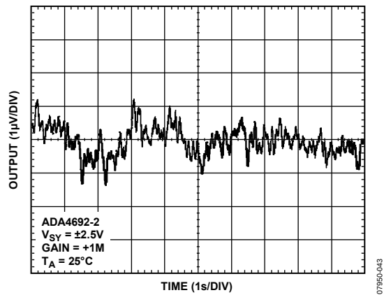
Figure 37. 0.1 Hz to 10 Hz Noise
