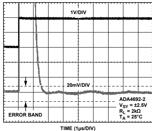
Figure 48. Positive Settling Time to 0.1%
