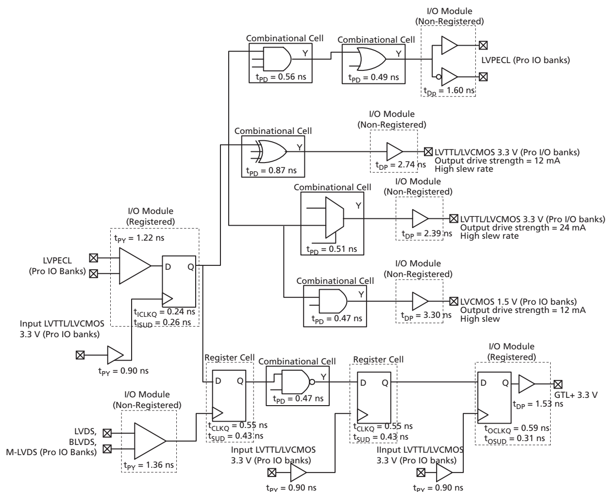
Figure 2-107 • Timing Model
