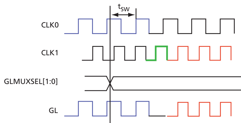
Figure 2-26 • NGMUX Waveform
