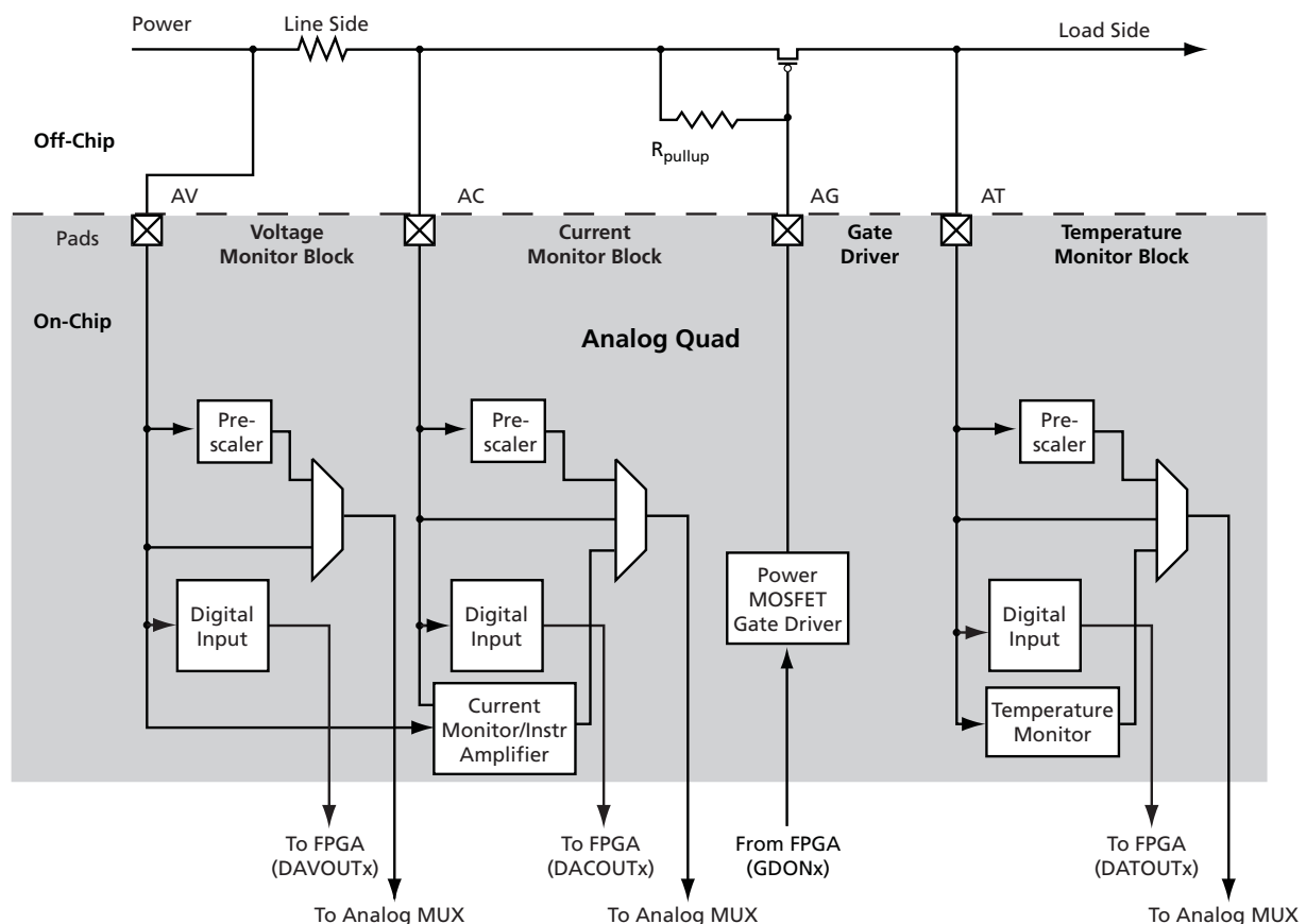
Figure 1-1 • Analog Quad
