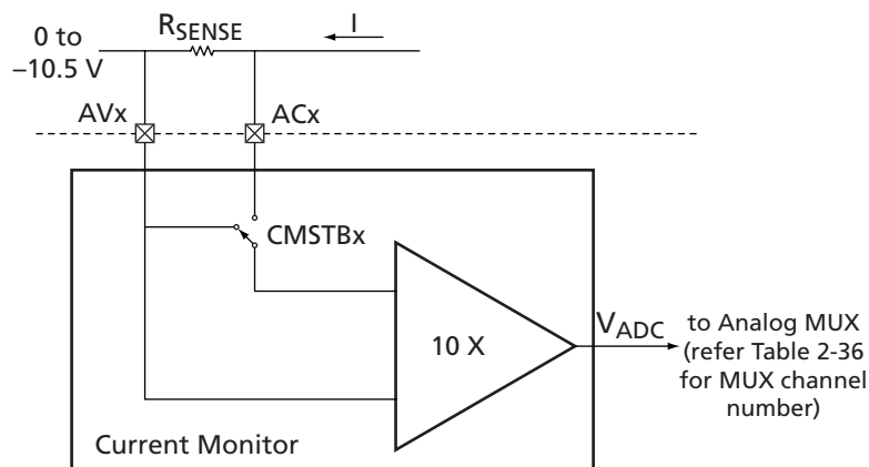
Figure 2-73 • Negative Current Monitor
