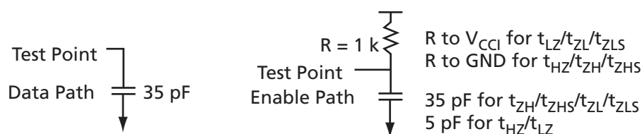
Figure 2-114 • AC Loading
