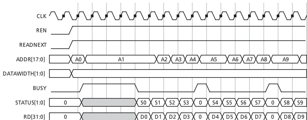
Figure 2-39 • Read Next Waveform (Non-Pipe Mode, 32-bit access)
