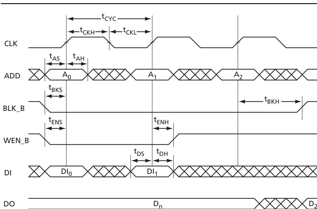
Figure 2-51 • RAM Write, Output Retained (WMODE = 0)
