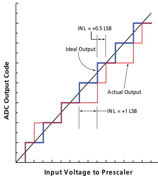
Figure 2-86 • Integral Non-Linearity (INL)
