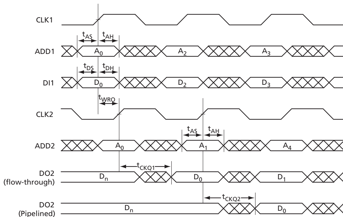
Figure 2-53 • One Port Write / Other Port Read Same
