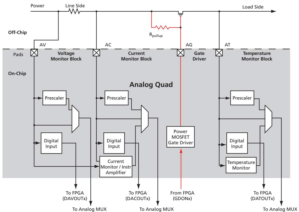
Figure 2-74 • Gate Driver
