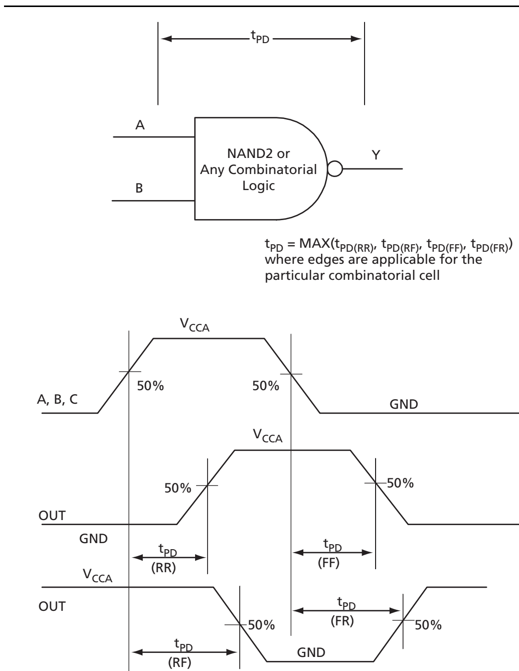
Figure 2-4 • Combinatorial Timing Model and Waveforms
