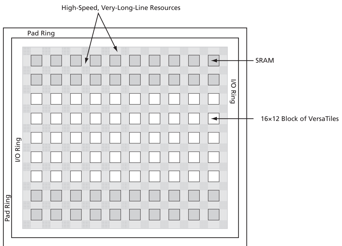
Figure 2-10 • Very-Long-Line Resources
