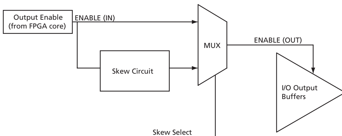
Figure 2-99 • Block Diagram of Output Enable Path
