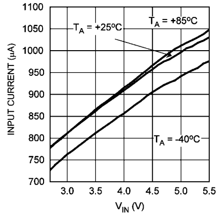
Switching Supply Current vs. V_{IN}
