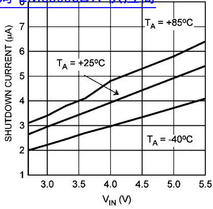
Shutdown Current vs. V_{IN} 查询"LM3509SDX"供应商
