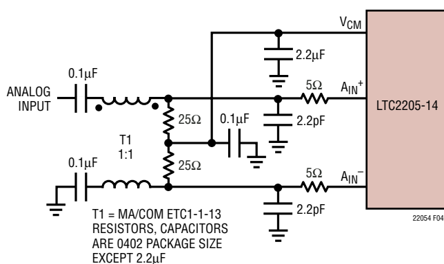
Figure 4b. Using a Transmission Line Balun Transformer. Recommended for Input Frequencies from 250MHz to 500MHz
