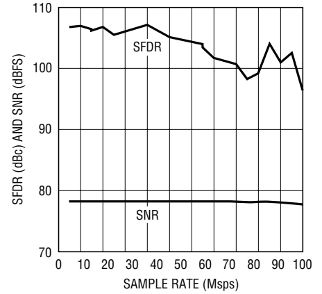
LTC2205-14: SFDR and SNR vs Sample Rate, f_{IN} = 5.1\text{MHz} , RAND = 0, DITH = 0
