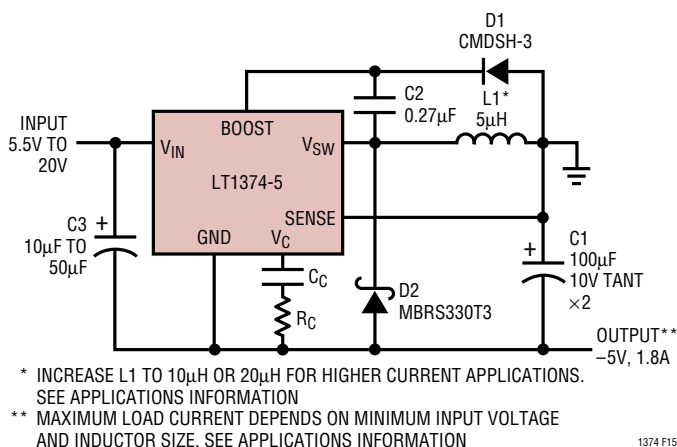
Figure 15. Positive-to-Negative Converter
