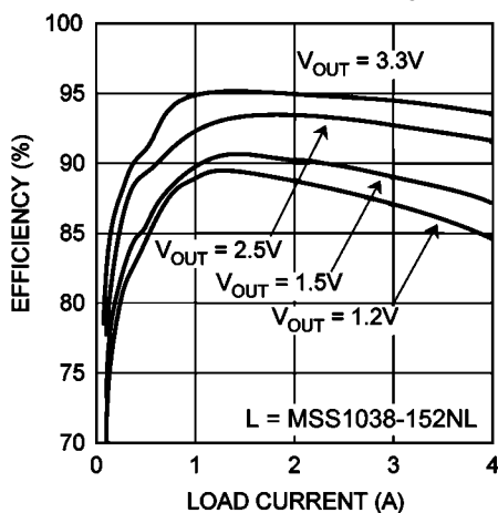
Efficiency vs. Load Current ( V_{IN} = 5\text{V} , f_{SW} = 500 \text{ kHz} )
