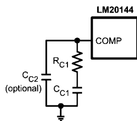
FIGURE 5. Compensation Network for LM20144
