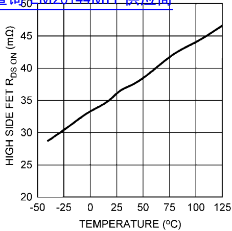
High-Side FET Resistance vs. Temperature 查询"LM20144MH"供应商
