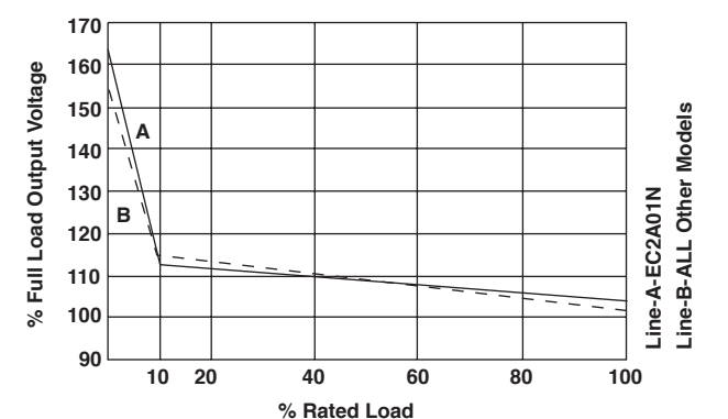
Typical Load Regulation
