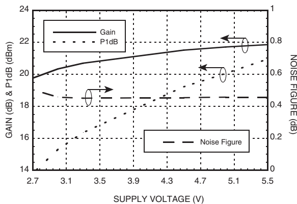
Gain, Power & Noise Figure vs. Supply Voltage @ 400 MHz
