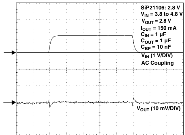
200 μS/DIV Line Transient Response
