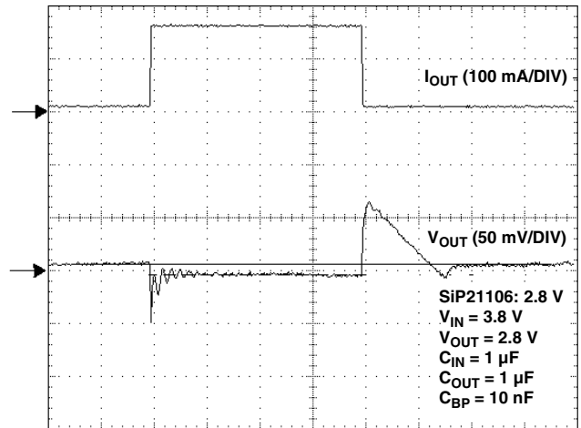
50 μS/DIV Load Transient Response
