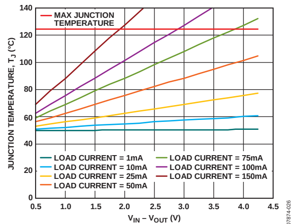
Figure 35. 0 mm 2 of PCB Copper, T_A = 50^\circ\text{C}
