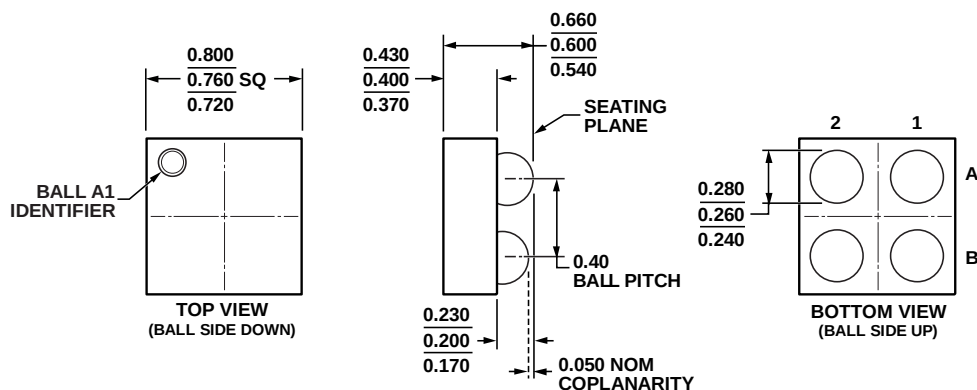
Figure 39. 4-Ball Wafer Level Chip Scale Package [WLCSP] (CB-4-3)
