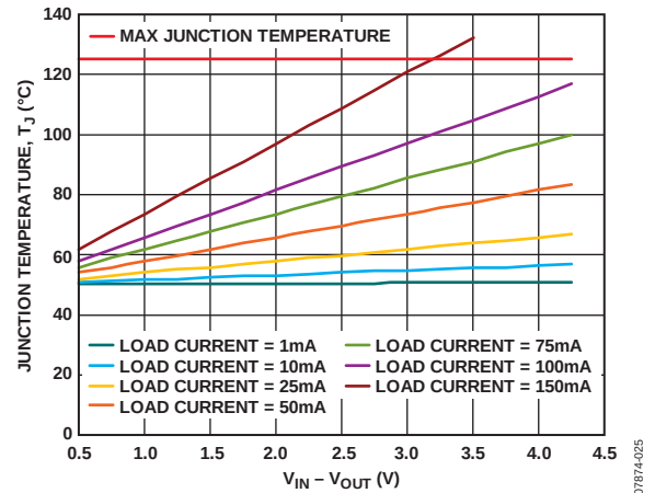
Figure 34. 100 mm 2 of PCB Copper, T_A = 50^\circ\text{C}
