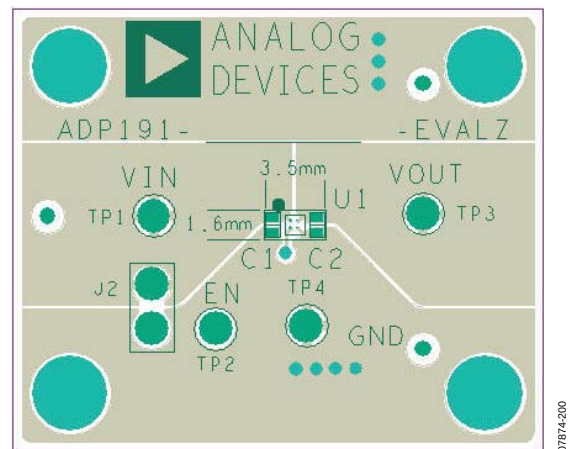
Figure 38. ADP191 PCB Layout
