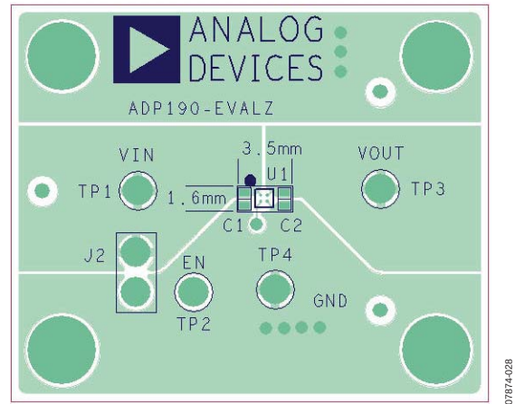
Figure 37. ADP190 PCB Layout
