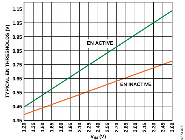
Figure 22. Typical EN Pin Thresholds vs. Input Voltage, V_{IN}
