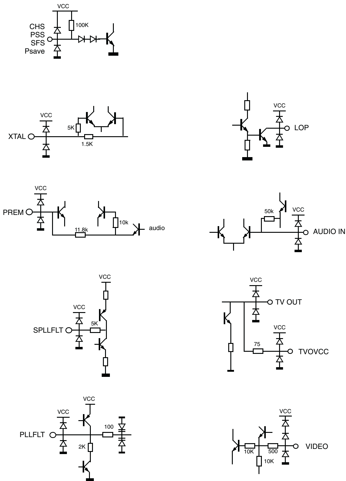
Figure 3. Pin Schematics
