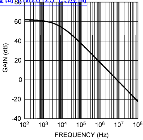
Error Amplifier Gain vs. Frequency 查询"LM20123"供应商
