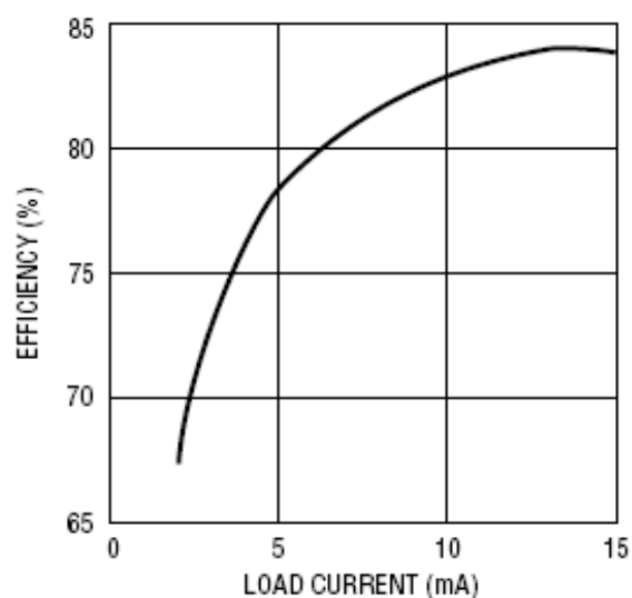
Seven LED Efficiency
