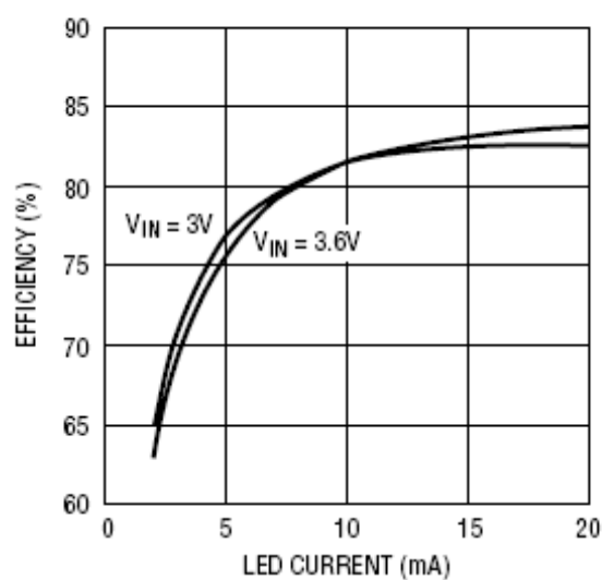
Three LED Efficiency
