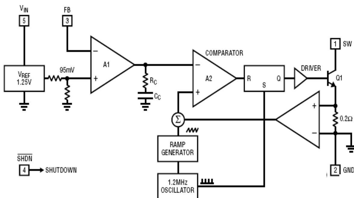
Figure 1. SM8237 function block diagram
