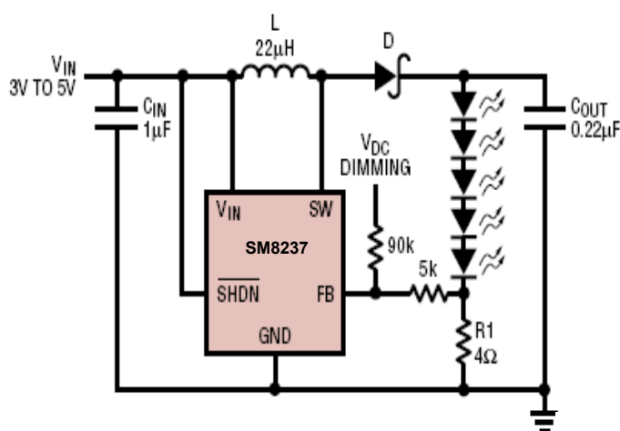
Li-Ion to Five White LEDs
